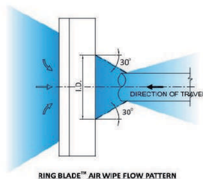
RING BLADE™ AIR WIPE FLOW PATTERN
